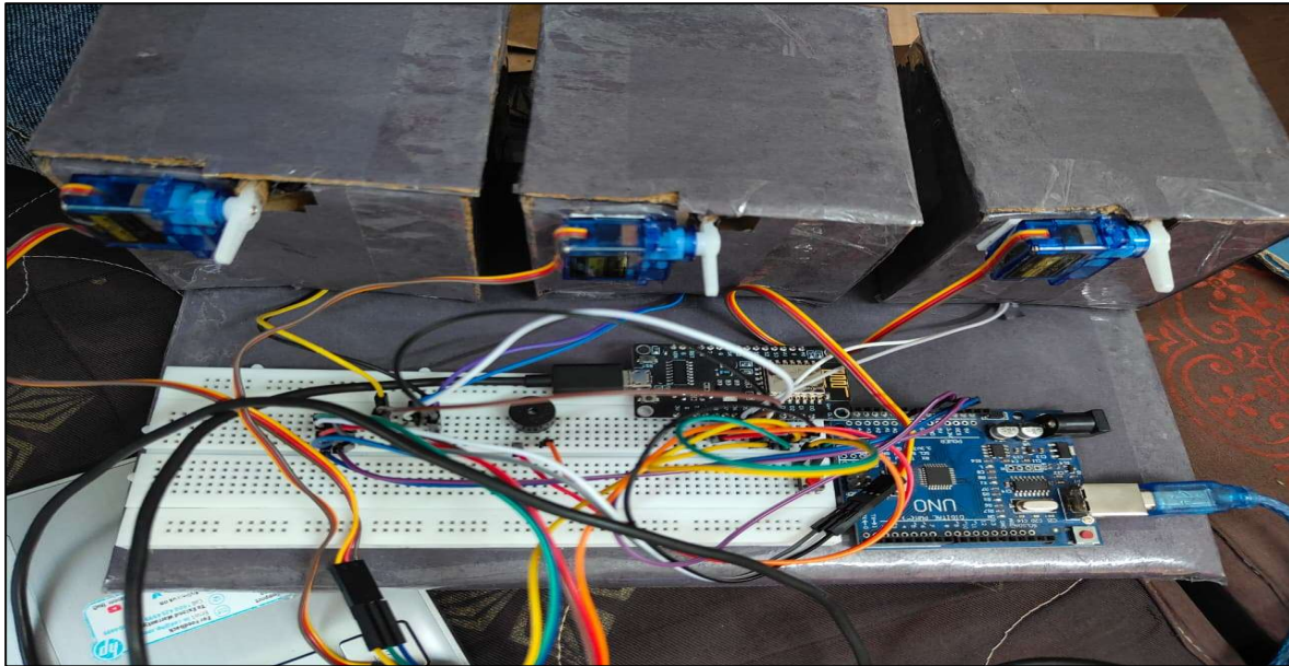
Figure 5 : Hardware Model
